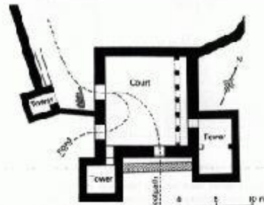
Fig. 69. PERGAMON. Estimated plan of main entrance.
